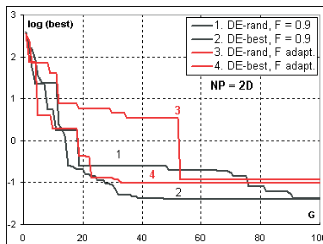
Fig. 2: Development of convergence in population NP = 2D
