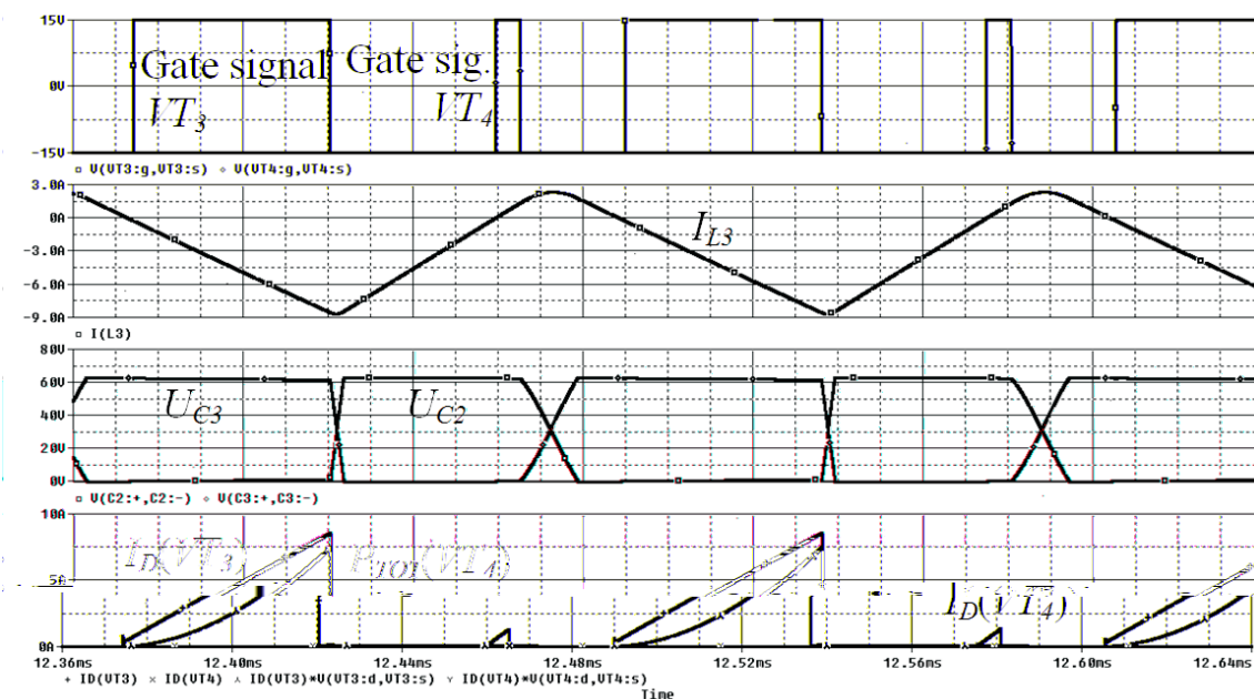
Fig. 9: Simulation results for output two-quadrant boost converter with ZVS; regeneration mode
