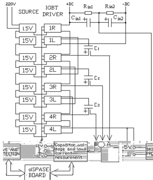
Fig. 7: Structural scheme of the experimental model of a single-phase five-level flying capacitor inverter
