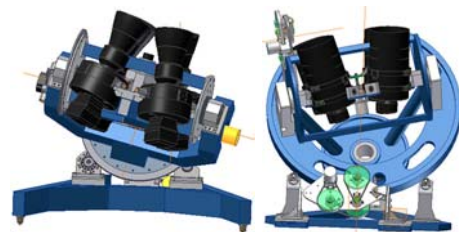
Fig. 4: Mount design with 2 CCD cameras (prototype in Chile)(left) and for 4 CCD cameras (new detector unit in Spain) (right)
