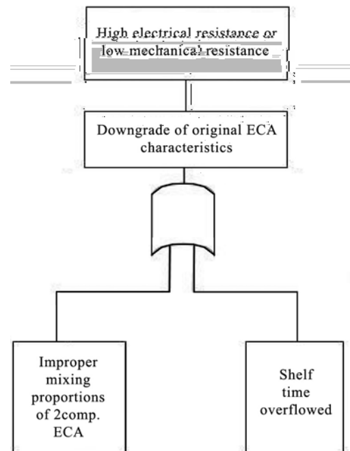
Fig. 5: FTA for joints formed by ECA
