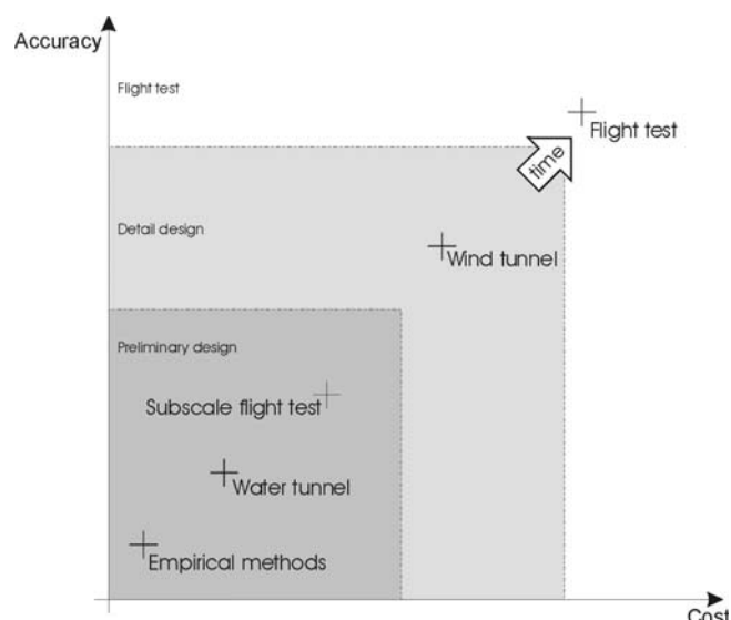
Fig. 6: Tradeoffs of accuracy and cost in methods selection
