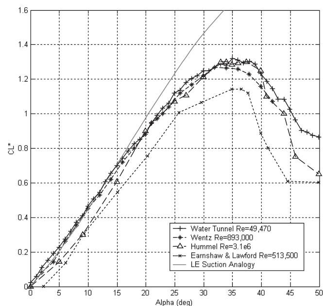
Fig. 4: Matching of force data for water and wind tunnel tests of a 65° delta wing
