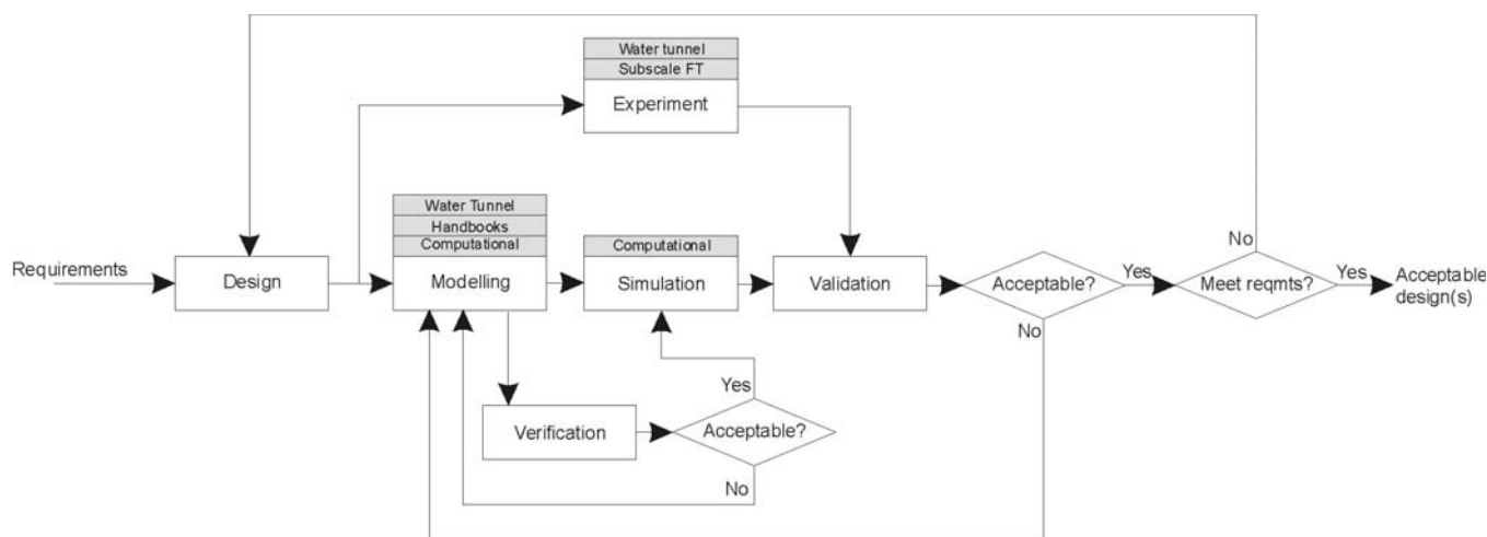
Fig. 3: Conceptual design process with physical and virtual modelling elements
