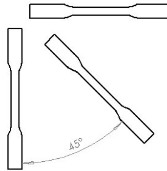
FIGURE 3. Orientation of the samples in the workspace of the FDM device.
