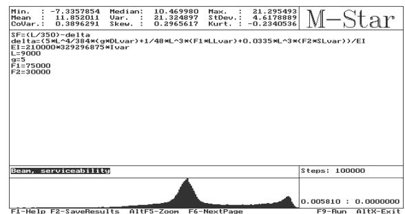
b) Reliability Analysis for Serviceability
