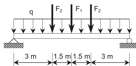
Fig. 3: Steel beam example
