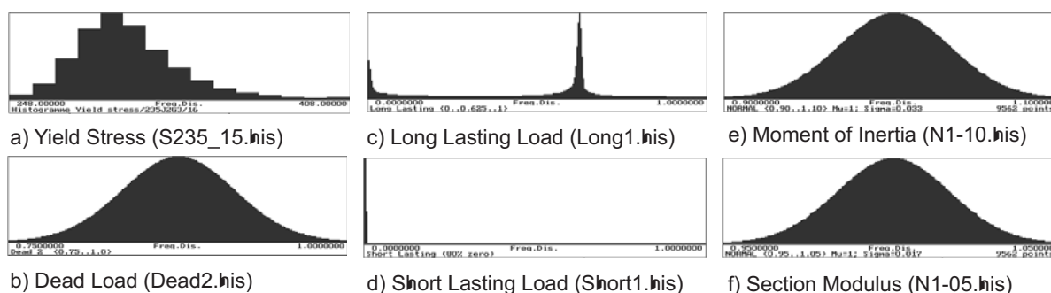
Fig. 4: Bounded histograms used to represent variable loads and properties
