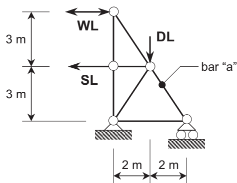
Fig. 6: Geometry of the example truss
