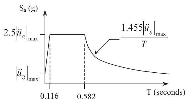
Spectrum 1. Structure on Stiff Soil Support
