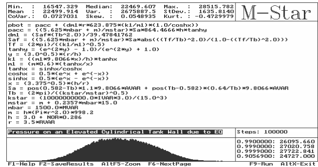
Fig. 12: Calculation of the maximum wall pressure using M-Star™
