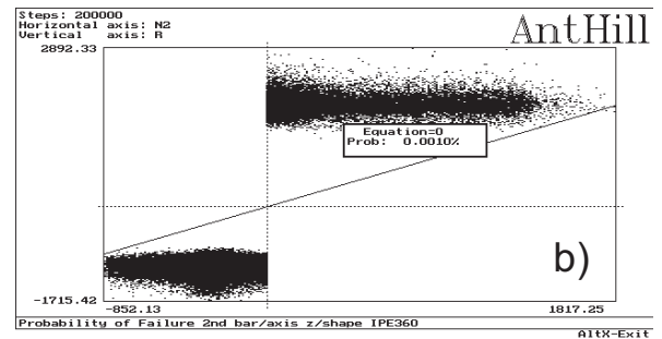
Fig. 9: Anthill™ program output: a) IPE330, b) IPE360
