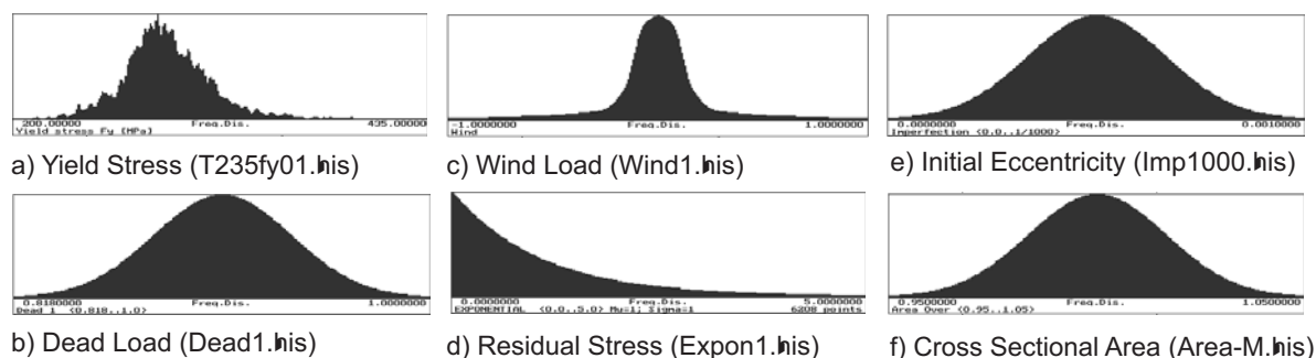
Fig. 7: Bounded histograms used to represent variable loads and variable properties
