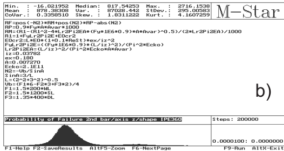
Fig. 8: M-Star™ program output: a) IPE330, b) IPE360
