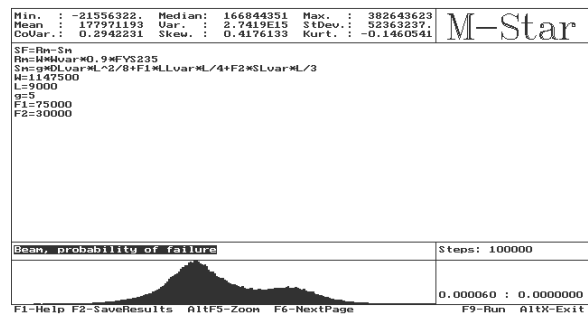
a) Reliability Analysis for Safety
