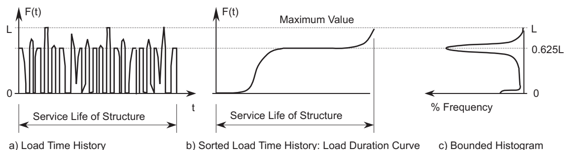
Fig. 1: Generation of load duration curve and corresponding bounded histogram for long lasting load
