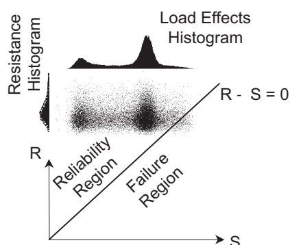
Fig. 2: Graphical representation of simulation based reliability assessment
