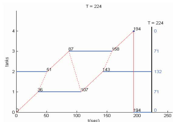
Fig. 2: Special chart for hoist scheduling
