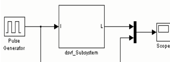
Fig. 4: Output Simulink scheme
